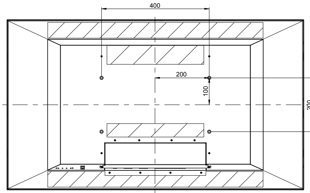
CuratOR LX491W / LX490W Unit : mm
